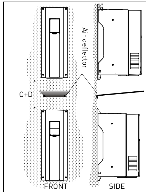
Figure 16. Installation space when drives are mounted on top of each other
