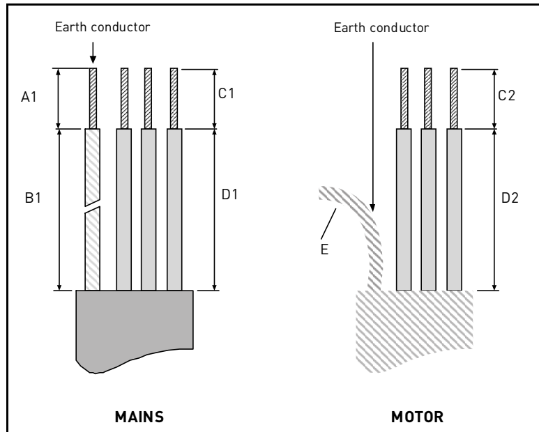
Figure 29. Stripping of cables
