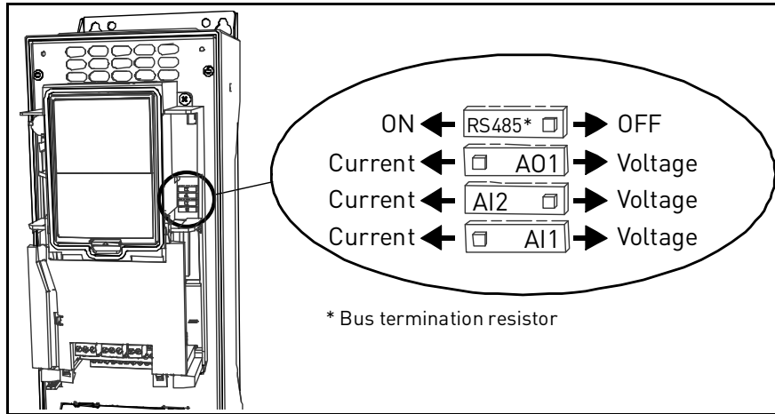
Figure 47. Dip switches
