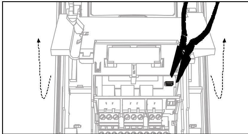
Figure 48. Remove this jumper to isolate the digital inputs from ground.
