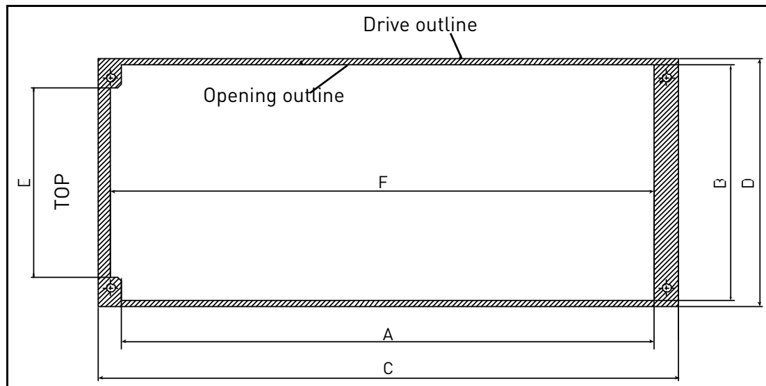
Figure 11. Flange mount cutout dimensions for MR4 to MR6
