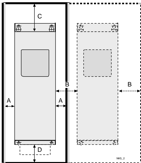
Figure 15. Installation space
