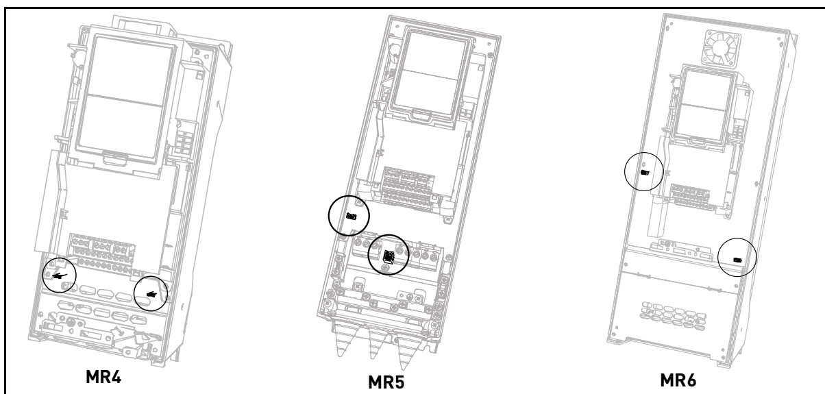
Figure 56. Locations of the EMC-jumpers in frames MR4 to MR6
