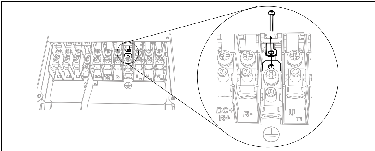
Figure 60. MR7: Detaching the DC grounding busbar from frame
