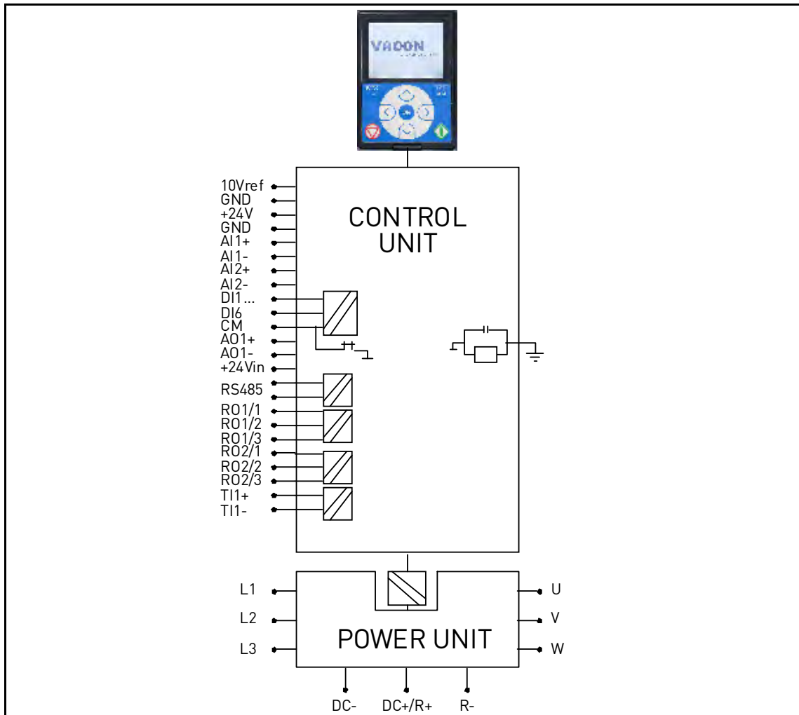
Figure 55. Galvanic isolation barriers
