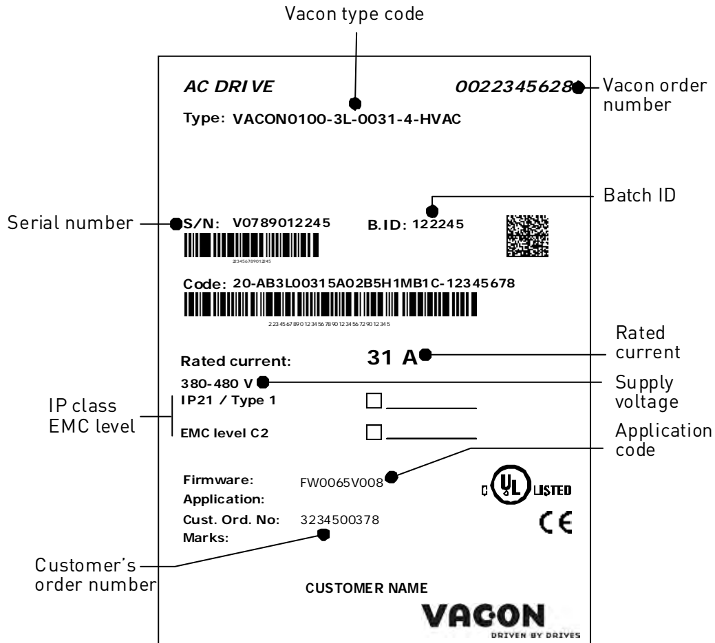
Figure 1. Vacon package label
