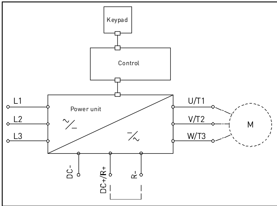
Figure 17. Principal connection diagram
