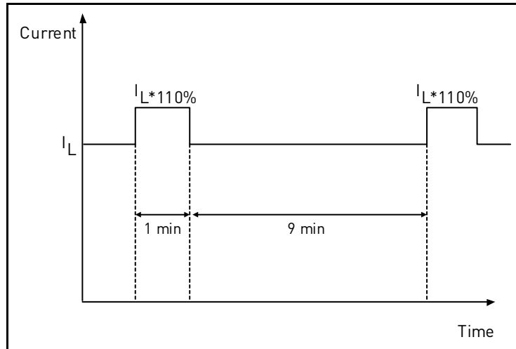
Figure 63. Low overload
