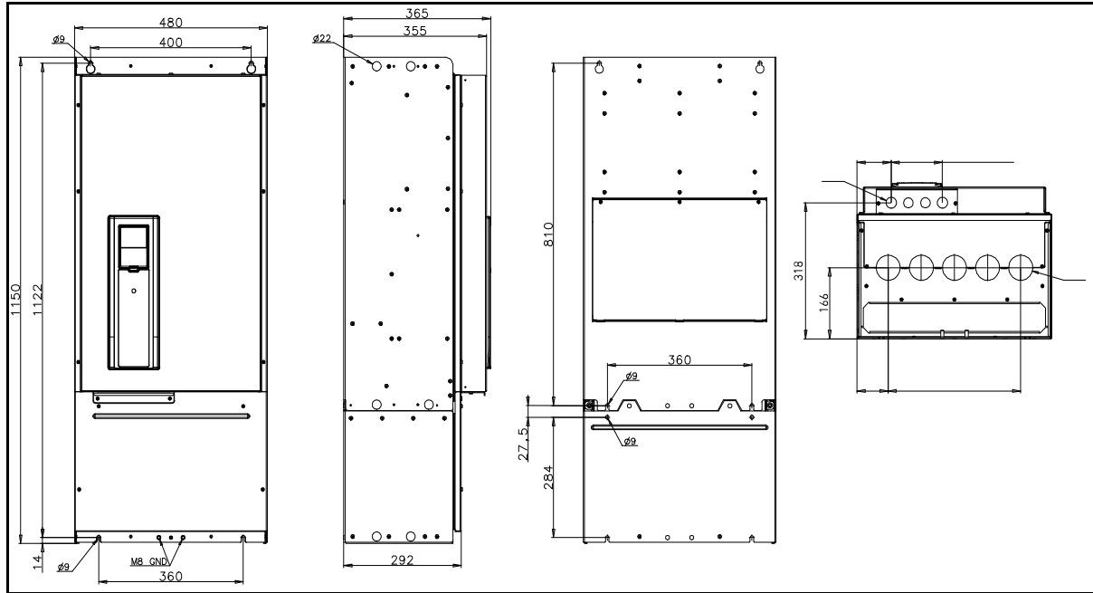
Figure 9. Vacon AC drive dimensions, MR9 IP21 and IP54
