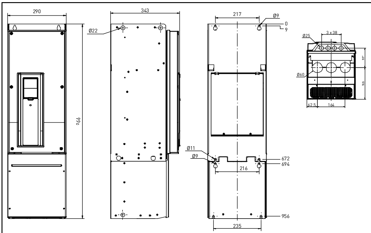
Figure 8. Vacon AC drive dimensions, MR8 IP21 and IP54
